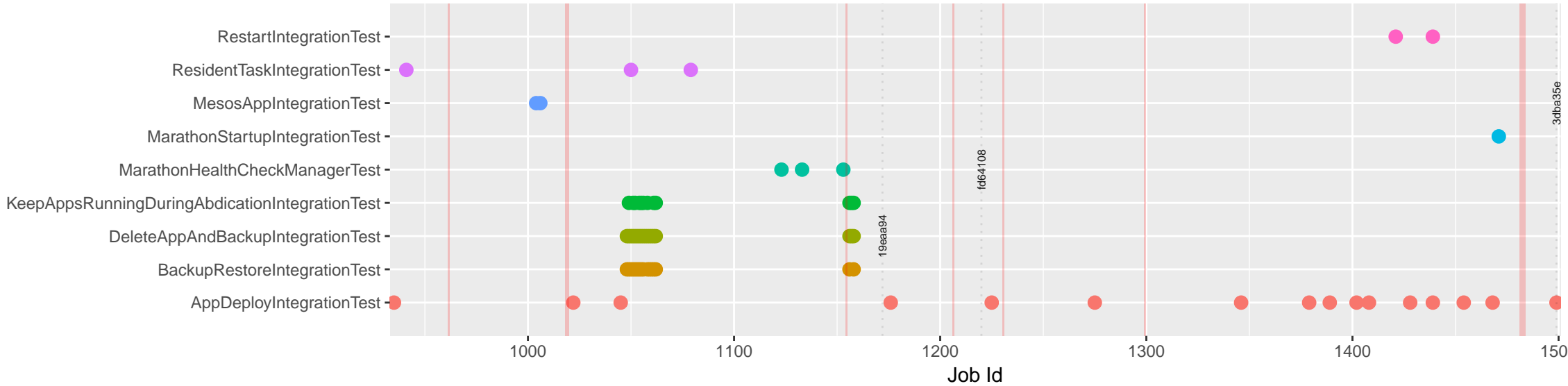
Failed suites for marathon-sandbox/job/marathon-loop-1.5 by Job (circle indicates failure)
